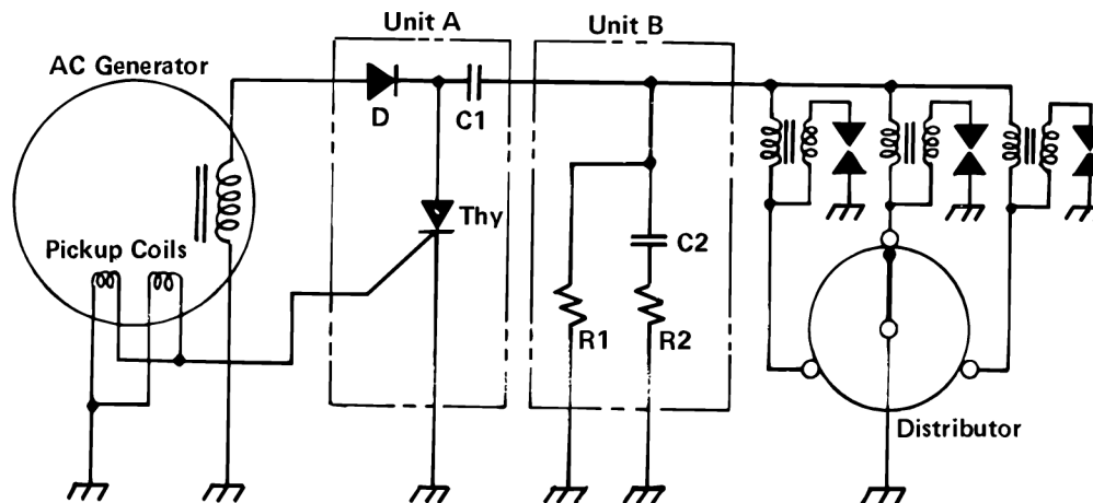
Ignition Circuit
